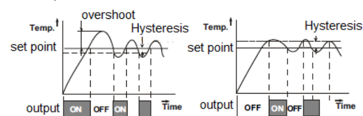
Figure 1.1: Typical Relay operation
