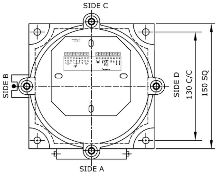
INTERNAL VIEW WITH TERMINAL CONNECTION DETAILS
