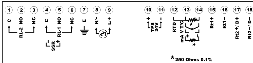
Figure 4.1: Terminal connection
