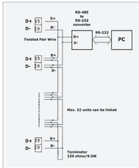
Fig 4.2: RS485 Connection Details
