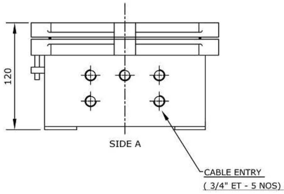
BOTTOM VIEW FOR CABLE ENTRY
