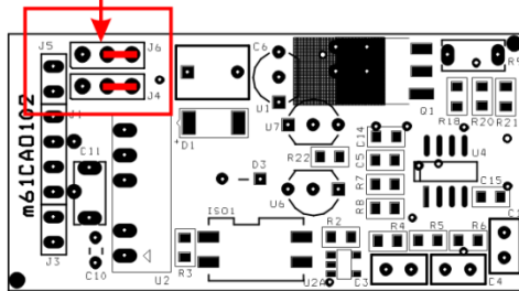
Jumper Settings for Current Output
