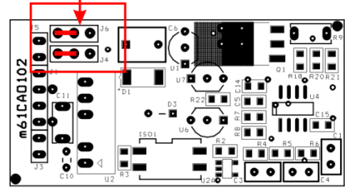
Jumper Settings for Voltage Output
