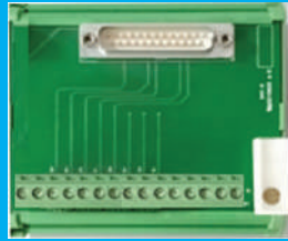
MAS-P-D25-M/MAS-P-D25-F D-Sub (PLC Side) to Screw Terminals (Field Side)
