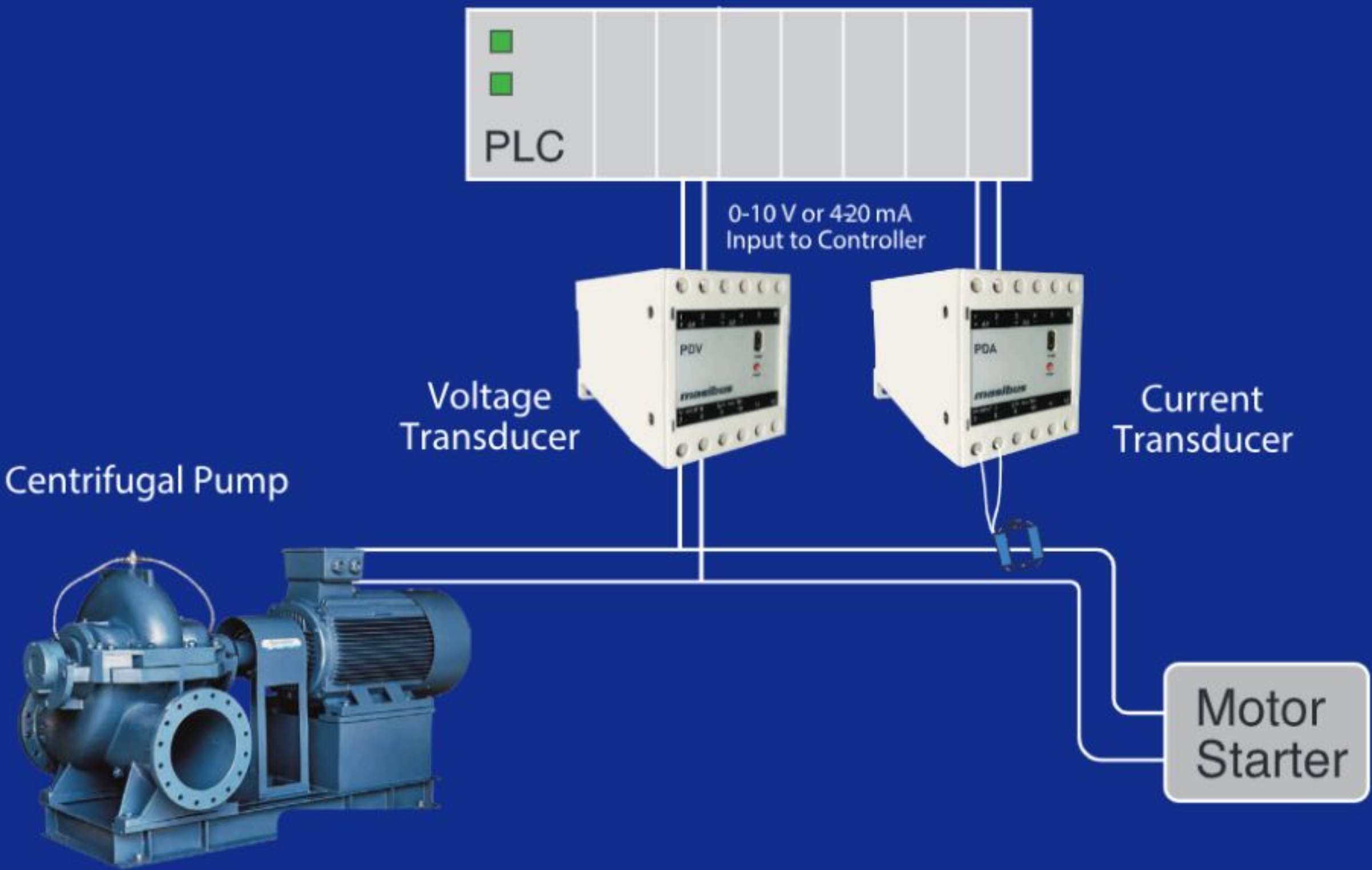
CURRENT MONITORING FOR SPIN PUMP APPLICATION
