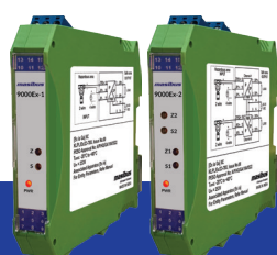
9000Ex-1/9000Ex-2 (One/ Two Channel Intrinsically Safe Transmitter Power Supply/ Isolated Barrier/ Signal Isolator)
