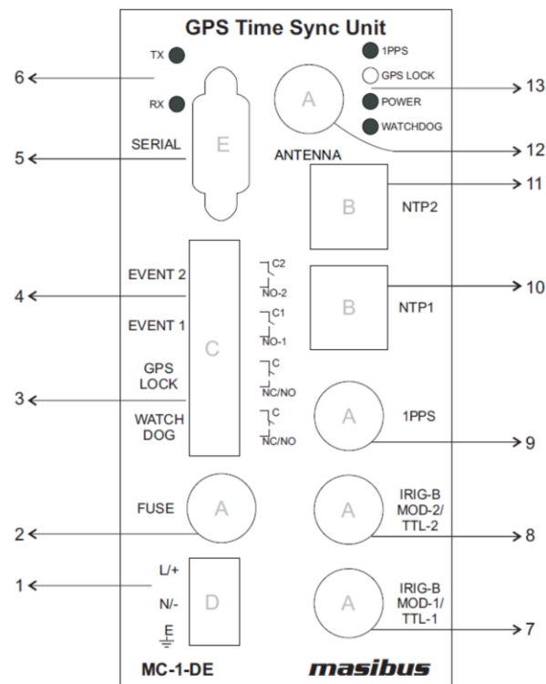
Figure 2 GPS Time Sync Unit Model MC-1-DE Front Panel
