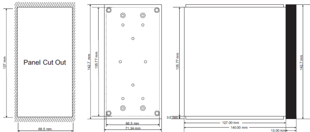
Figure 17 Panel Mount Mechanical Dimension Layout
