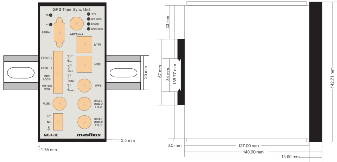
Figure 17 Din Rail Mount Mechanical Dimension Layout
