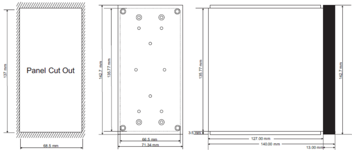
Figure 16 Panel Mount Mechanical Dimension Layout
