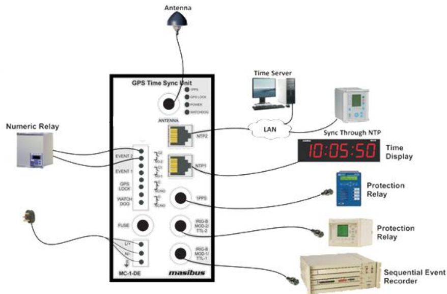
Figure 18 Wiring Diagram of GPS Time Sync Unit
