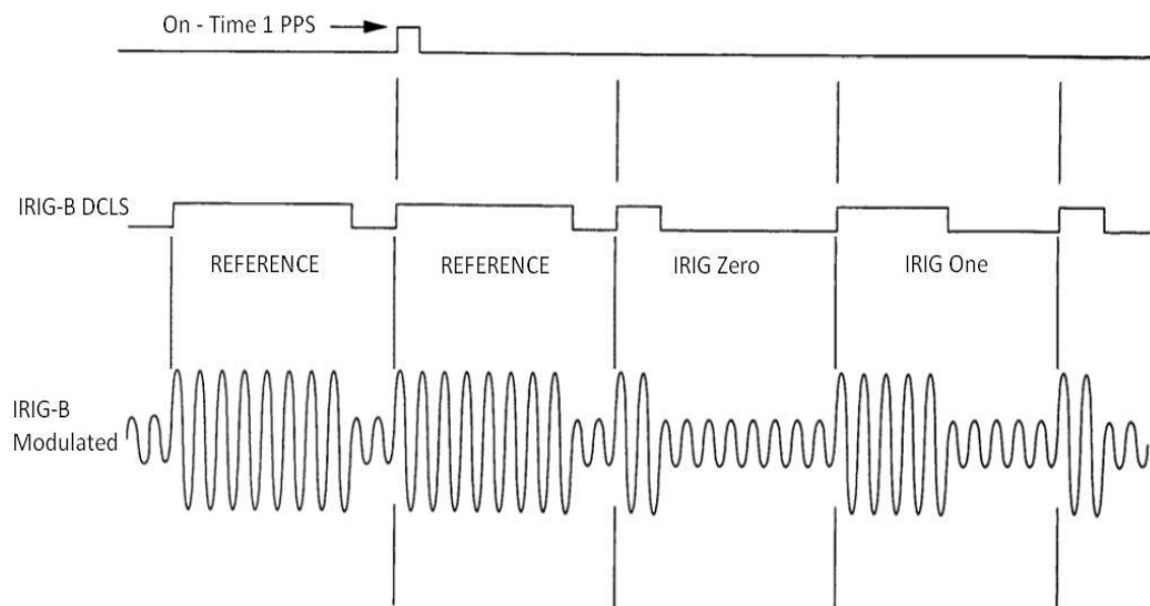
Figure 19 IRIG B Waveform
