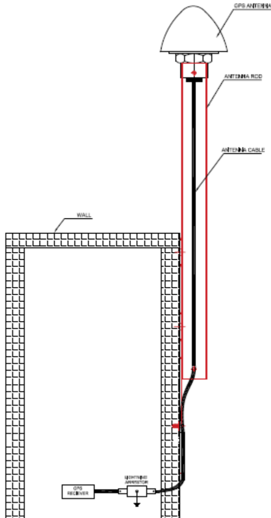
Figure 14 Antenna Mounting with Lightning Arrester
