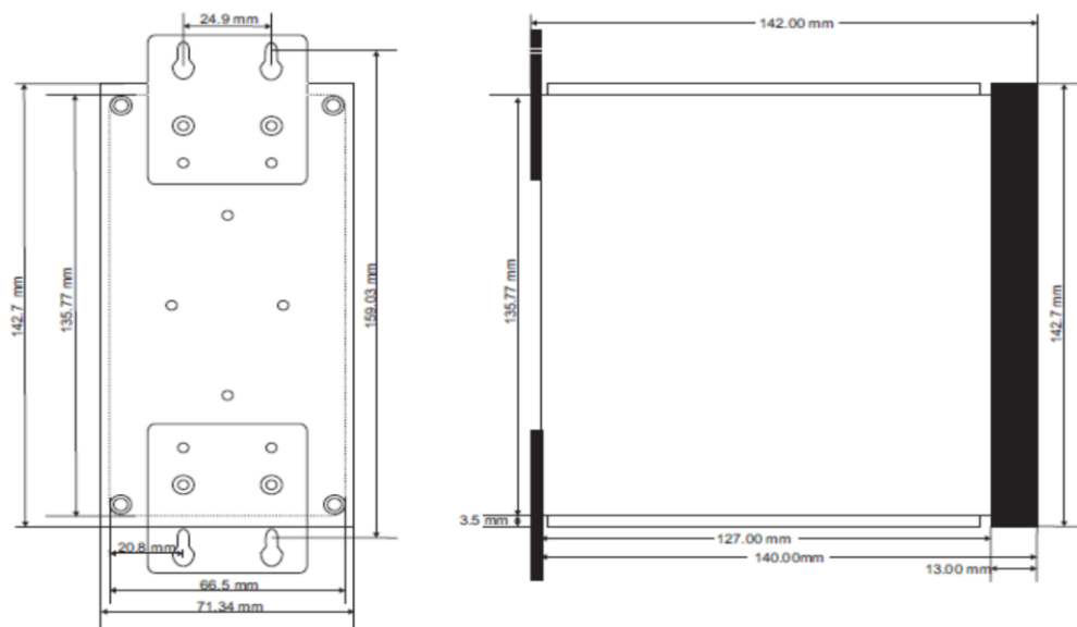
Figure 15 Wall Mount Mechanical Dimension Layout
