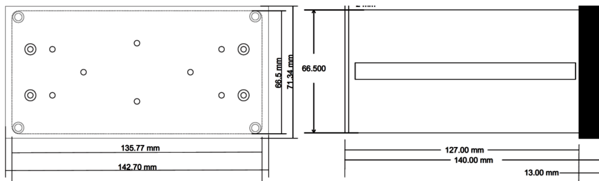
Figure 15 MC-1-DH Panel Mount-1
