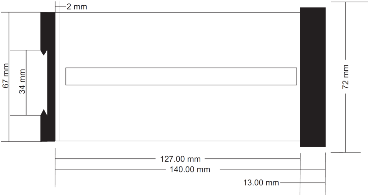
Figure 13 MC-1-DH Din rail Mount - 2
