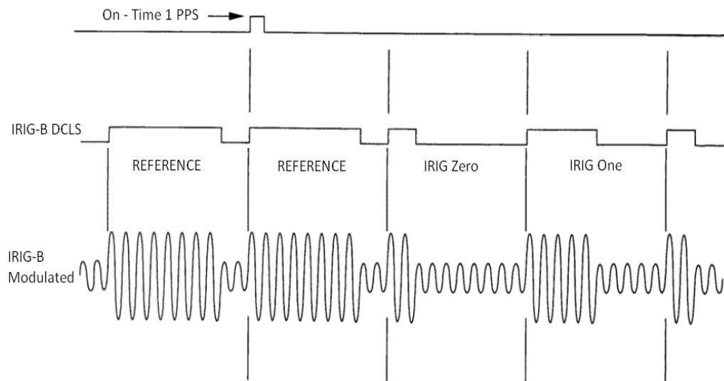
Figure 21 IRIG-B Waveform
