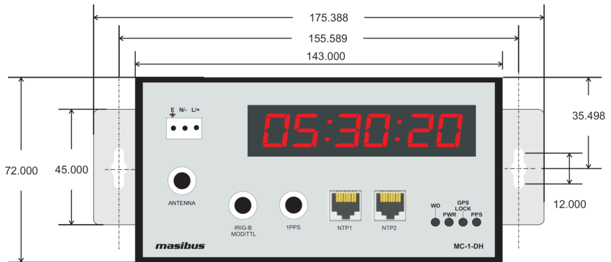
Figure 14 MC-1-DH Wall Mount
