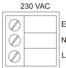
Figure 6 : Power Supply Connections
