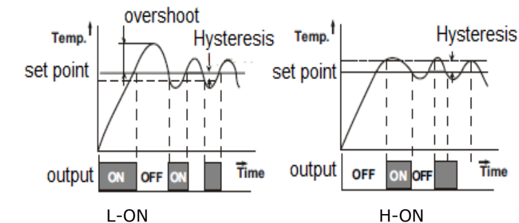
Figure 1.1: Typical Relay operation
