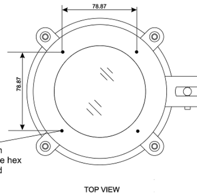
TOP VIEW FOR DISPLAY CARD ASSEMBLY
