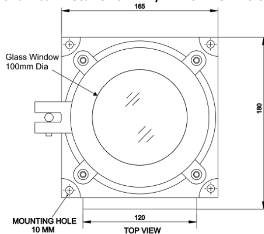
FRONT VIEW OF DEVICE
