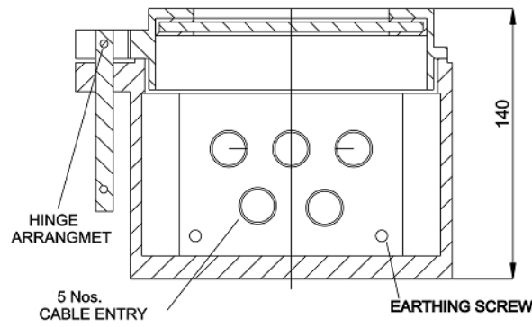
BOTTOM VIEW FOR CABLE ENTRY
