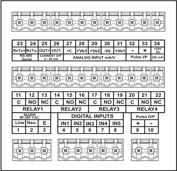
Terminal Details of 1008S Standard
