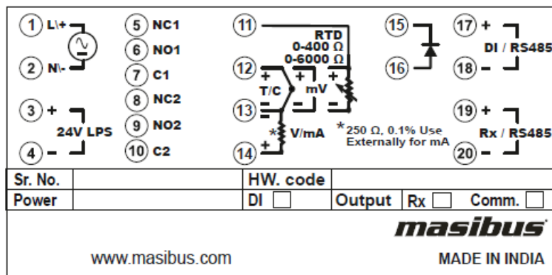
Fig 3. Terminal arrangement for 409
