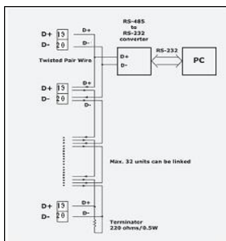
Fig 4.2: RS485 Connection Details
